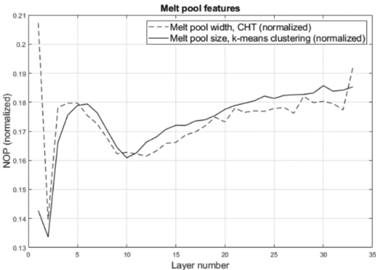
Fig. 5. Melt pool features extracted using CHT and K-means clustering techniques for image segmentation
